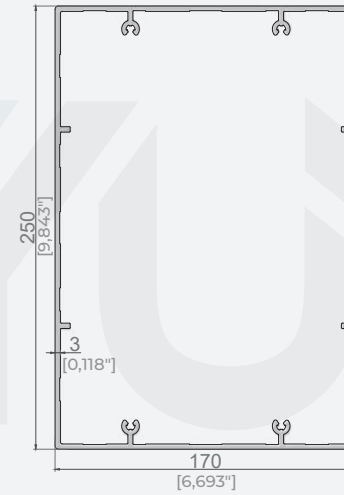
250x170 DİKME PROFİLİ 250x170 PILLAR PROFILE
