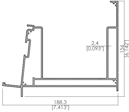
188,3x156 Düz Dere 188,3x156 Gutter Profile
