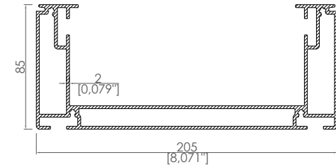
Dere Profili Gutter Profile
