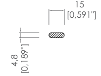
Alt Ray Teker Profili Bottom Rail Wheel Profile
