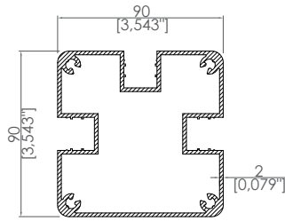
Standart Dikme Profili Standart Pillar Profile
