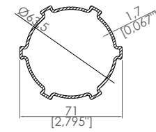
Motor Borusu Eki Motor Tube Connection
