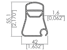
42x55,1 Kumaş Profili 42x55,1 Fabric Support Profile
