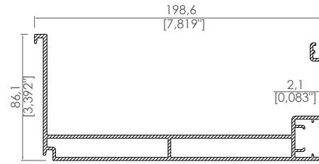
Dere Profili Gutter Profile
