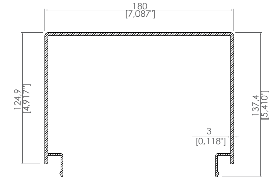
Dikme Kapak Profili Pillar Cover Profile
