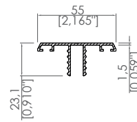
Orta Cam Kapak Profili Middle Glass Cover Profile
