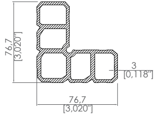
Cam Panel Köşe Takoza Glass Panel Corner Block Profile
