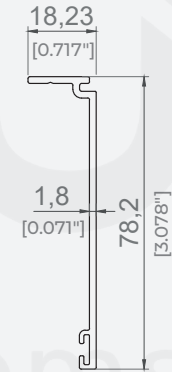
Yan Ray Kapak Profili / Side Rail Cover Profile
