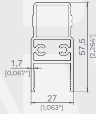
22MM CAM PANEL YAN PROFİL 22MM GLASS PANEL SIDE PROFILE
